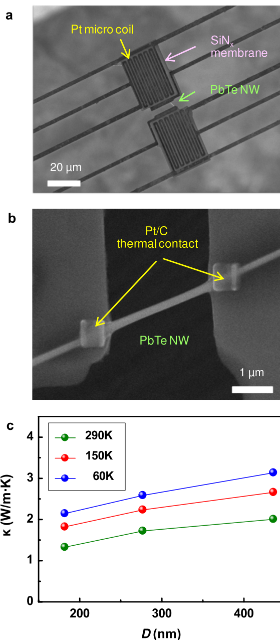
Figure 2. Thermal conductivity of individual PbTe nanowires. (a) An SEM image of a PbTe nanowire bridging two suspended heating membranes for thermal conductance measurement. (b) The highlighted SEM image of a thermal contact between the membrane and PbTe nanowire. (c) Diameter-dependent thermal conductivity of individual PbTe nanowires. The temperatures are 60, 150 and 290 K, respectively.
